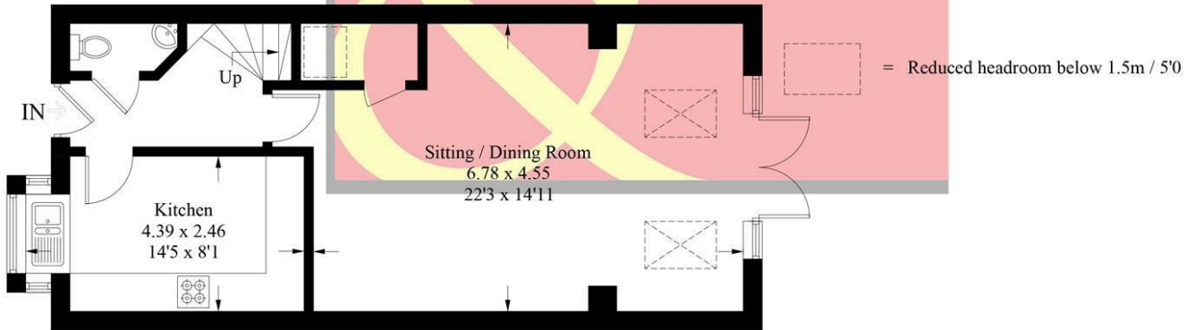
Ground Floor
